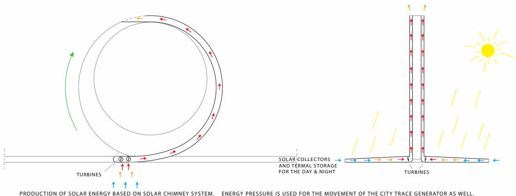
PRODUCTION OF SOLAR ENERGY BASED ON SOLAR CHIMNEY SYSTEM. ENERGY PRESSURE IS USED FOR THE MOVEMENT OF THE CITY TRACE GENERATOR AS WELL.
