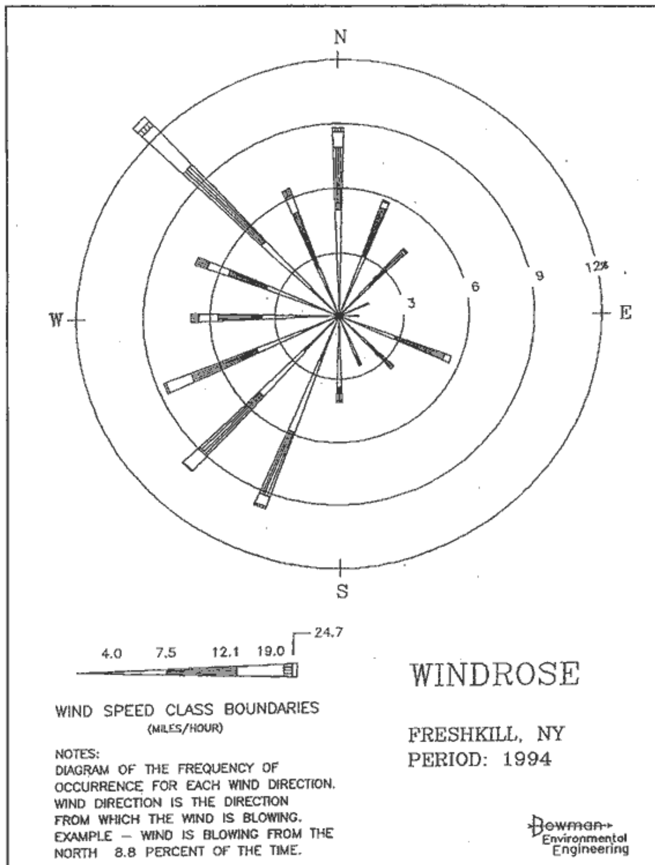
Figure 3 Example of prevailing wind directions: Windrose generated from meteorological data collected at the Fresh Kills Landfill in 1994
